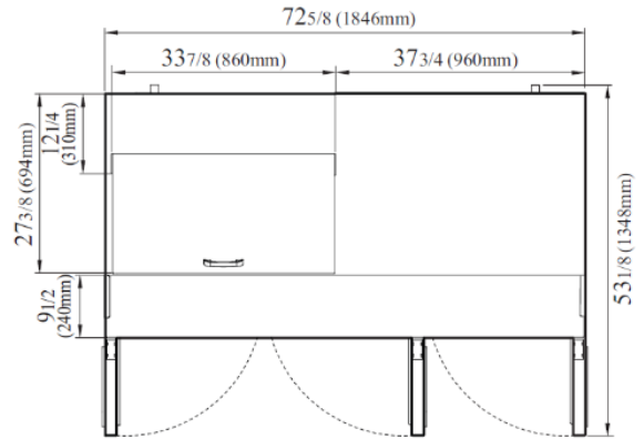
TST-72SD-15M-N VISTA SUPERIOR
