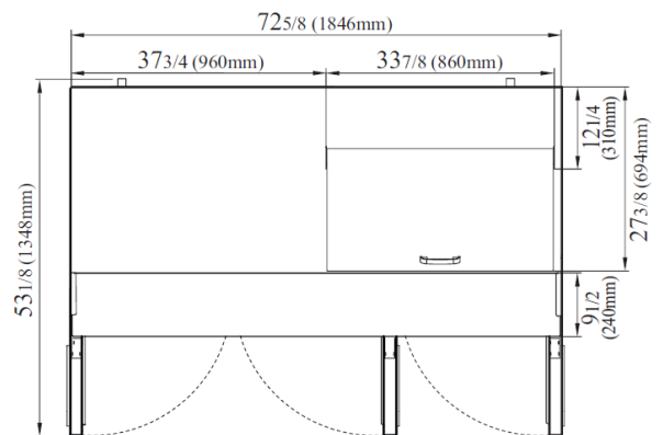
TST-72SD-15M-N-LW VISTA SUPERIOR
