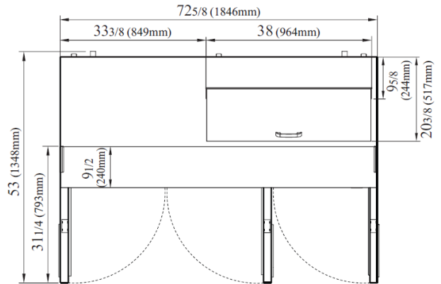
TST-72SD-10S-N-LW VISTA SUPERIOR
