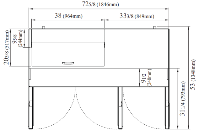
TST-72SD-10S-N VISTA SUPERIOR
