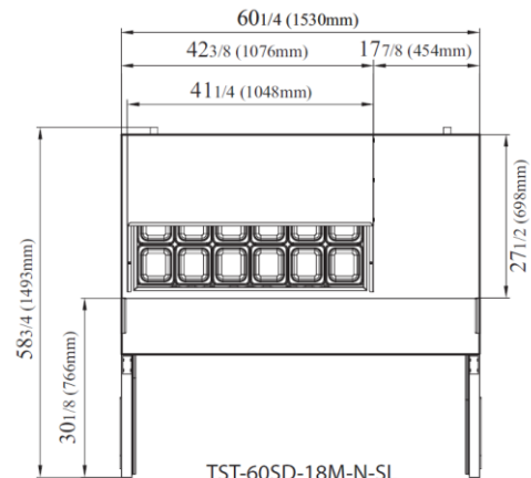
TST-60SD-18M-N-SL VISTA SUPERIOR
