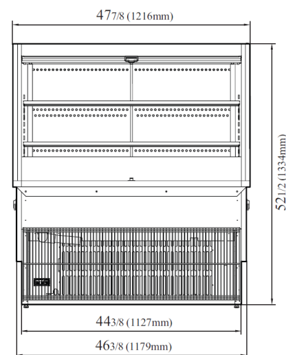
VISTA FRONTAL
