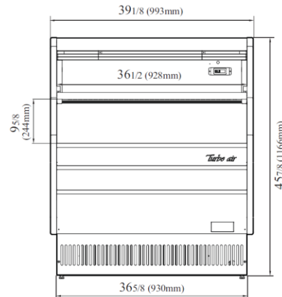
VISTA FRONTAL
