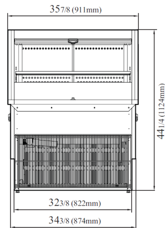
VISTA FRONTAL
