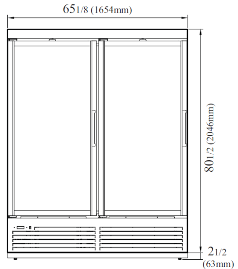
VISTA FRONTAL
