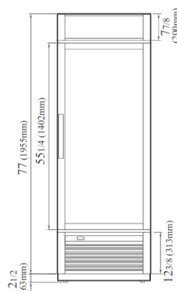
VISTA FRONTAL
