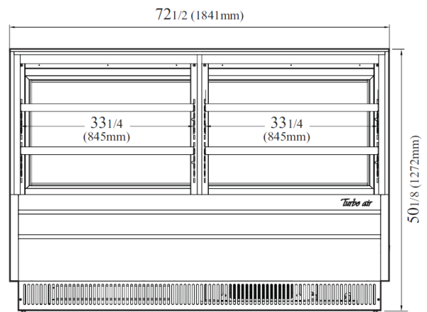
VISTA FRONTAL
