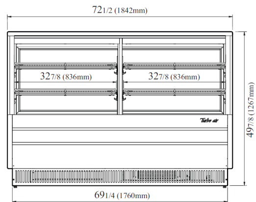
VISTA FRONTAL
