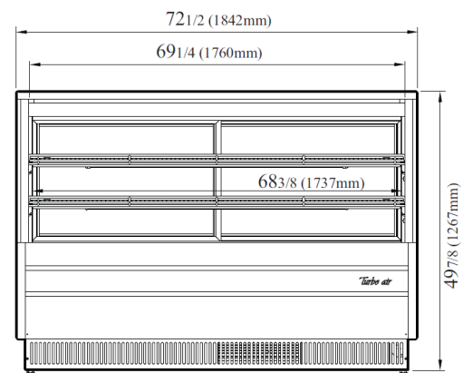
VISTA FRONTAL
