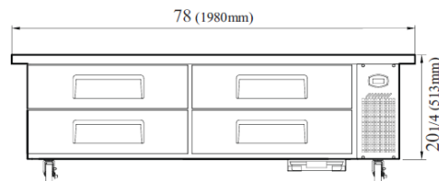
VISTA FRONTAL
