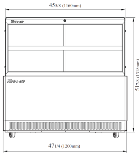
VISTA FRONTAL
