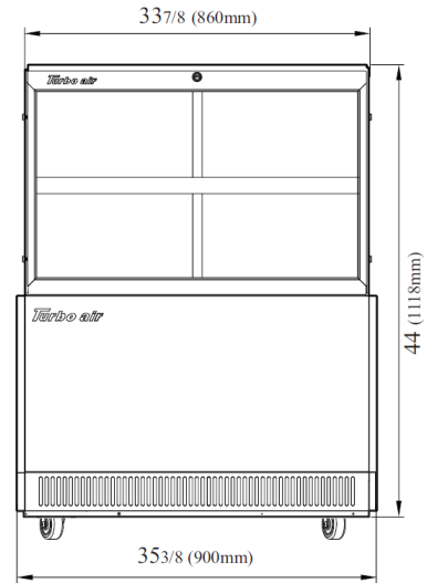
VISTA FRONTAL
