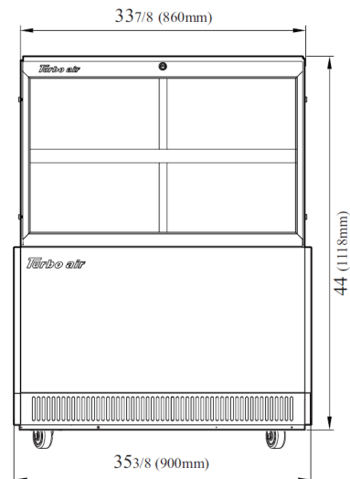
VISTA FRONTAL
