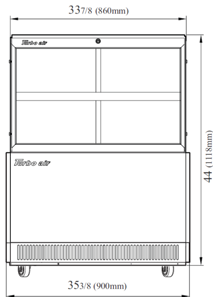
VISTA FRONTAL
