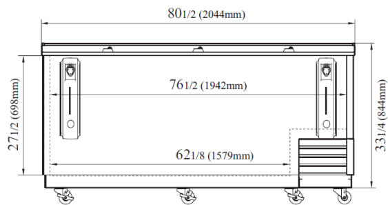
VISTA FRONTAL
