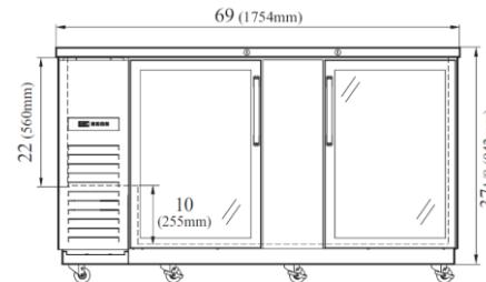
TBB-3SGD-N VISTA FRONTAL
