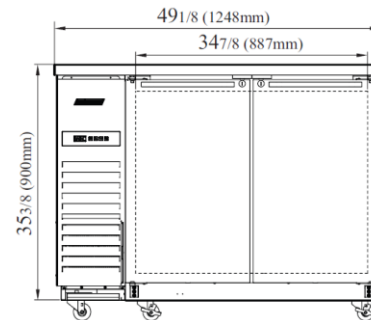
TBB-24-48SSD-N6 VISTA FRONTAL
