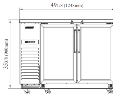
TBB-24-48SGSD-N VISTA FRONTAL
